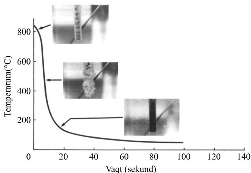
2-rasm. "Inconel 600" ni polialkilen glikol(PAG) toblash muhitida sovutish.
